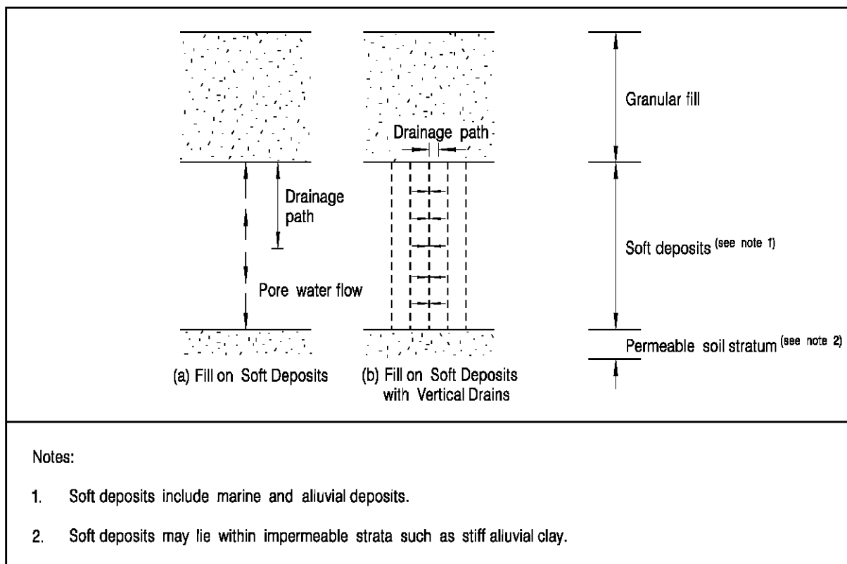
Figure 8 – Shortening of Drainage Path by Vertical Drains
